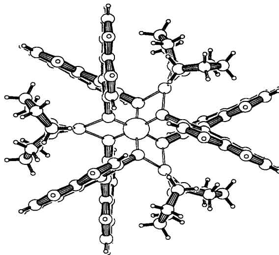
Figure 2. Molecular structure of AlLi 3 BINOL 3 ·6THF 6 .
